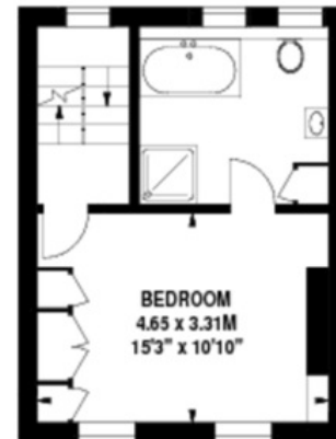
Second Floor 280 sq ft
